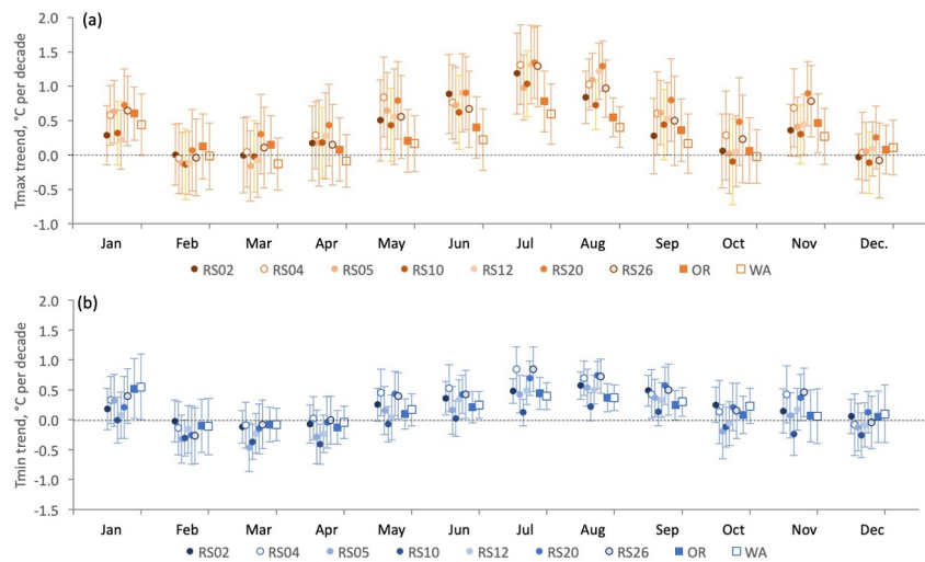
Figure 3. Rates of change of (a) mean monthly maximum air temperature ( T_{\max} ) and (b) mean monthly minimum air temperature ( T_{\min} ) ( ^{\circ}\text{C}/\text{decade} ) at reference stands in the Andrews Forest and for statewide average temperature at all USHCN stations in Oregon and Washington ( n = 84 ), 1979–2023. Error bars are the 95% confidence interval around the slope term from a linear regression. Symbol colors indicate low to high elevation, left to right, dark to light shades (see Table S2 in Supporting Information S1 reference stand site characteristics). Numbers in Table S3 in Supporting Information S1. Data sources: Daly et al. (2024), Menne et al. (2012), Office of the Washington State Climatologist (2024).
