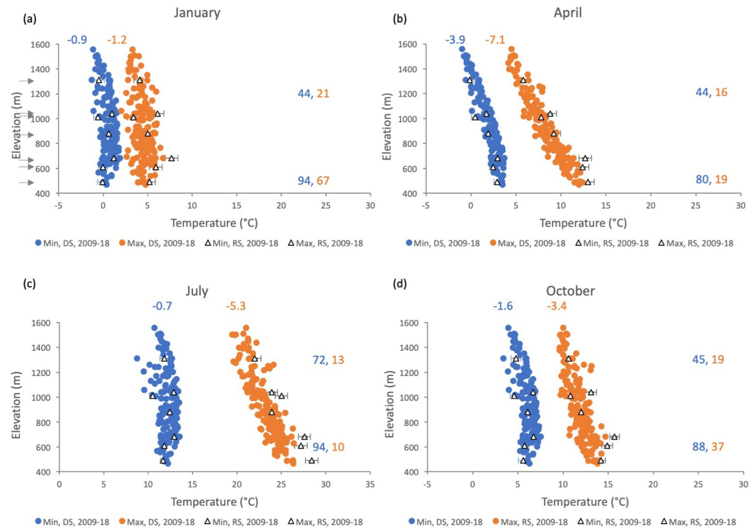
Figure 7. Average monthly T_{\min} (blue) and T_{\max} (orange), 2009–2018, at distributed temperature sensors (circles) and reference stands (open black triangles) in the forest understory (X axis) versus elevation (Y-axis) for (a) January, (b) April, (c) July, and (d) October. Values are mean \pm SE (sensor height 1.5 m). Arrows at left in (a) indicate elevations of the seven reference stands used for long-term trend analysis (Figure 3). Numbers at top are the temperature gradient with elevation ( ^{\circ}\text{C}/1,000\text{ m} ) based on linear models fitted to the 2009–2018 means (circles). Numbers to the right are the percent of hours of down-slope, down-valley winds during the night (first number) and during the day (second number) at near ridge (VAN, 1,268 m, Figure 2) and valley bottom (PRI, 436 m, Figure 2) meteorological stations from 2015 to 2018. Data sources: Schulze et al. (2023) and Daly et al. (2024).
