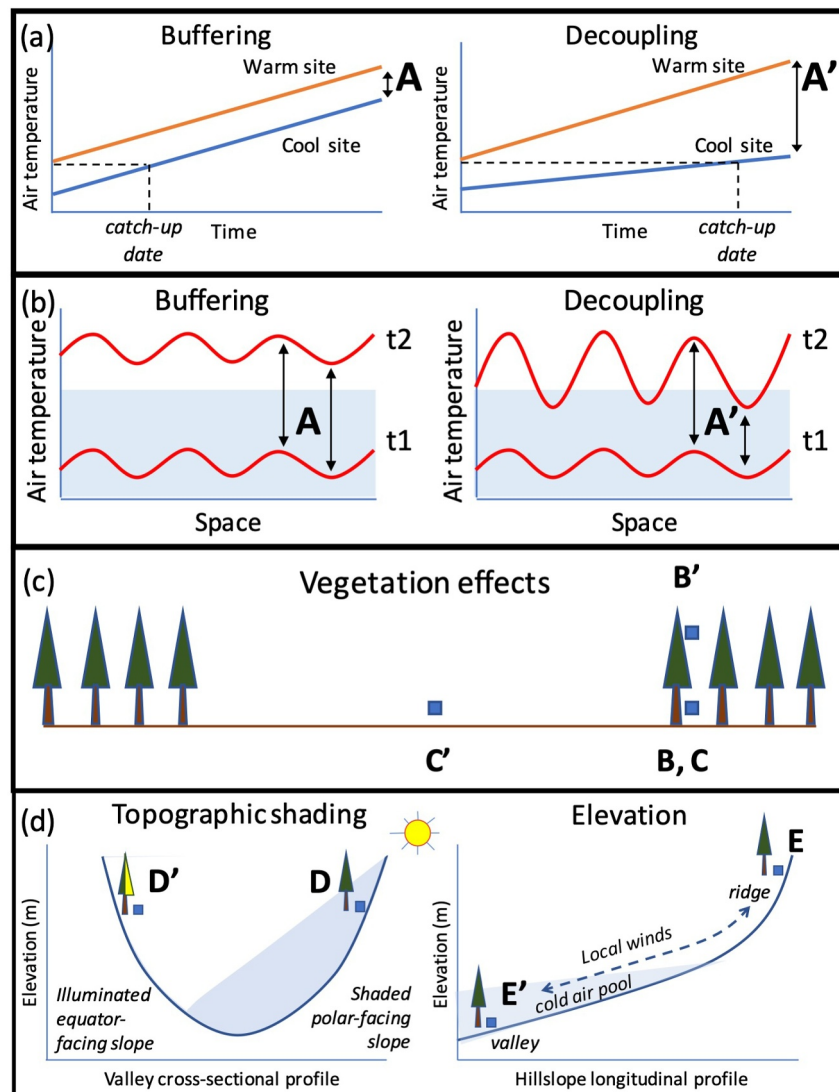
Figure 1. Concepts about temporal change in temperature and factors influencing spatial patterns of temperature. (a) Buffering ( A ) and decoupling ( A' ) in time. (b) Buffering ( A ) and decoupling ( A' ) in space, relative to some hypothetical tolerance limits (blue shading). (c) Vegetation effects produce differences between the forest canopy and the understory ( B' – B ) and between canopy openings and the forest understory ( C' – C ). (d) Effects of topography, that is, illuminated-versus shaded (blue shading) slopes ( D' – D ) and elevation, including air temperature decline as elevation increases and cold air pooling produced by local winds (blue shading) ( E' – E ).
