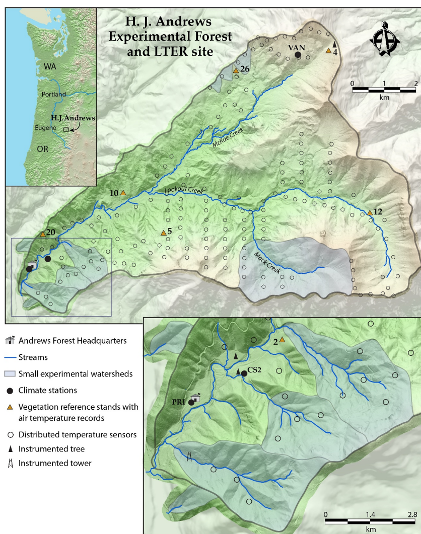
Figure 2. Location of the H.J. Andrews Experimental Forest and climate records used in this study, including meteorological stations, reference stands (numbered triangles), distributed temperature sensors (open circles), vertically instrumented trees (black triangles), and instrumented tower (See Table S1 in Supporting Information S1 for data set characteristics).
