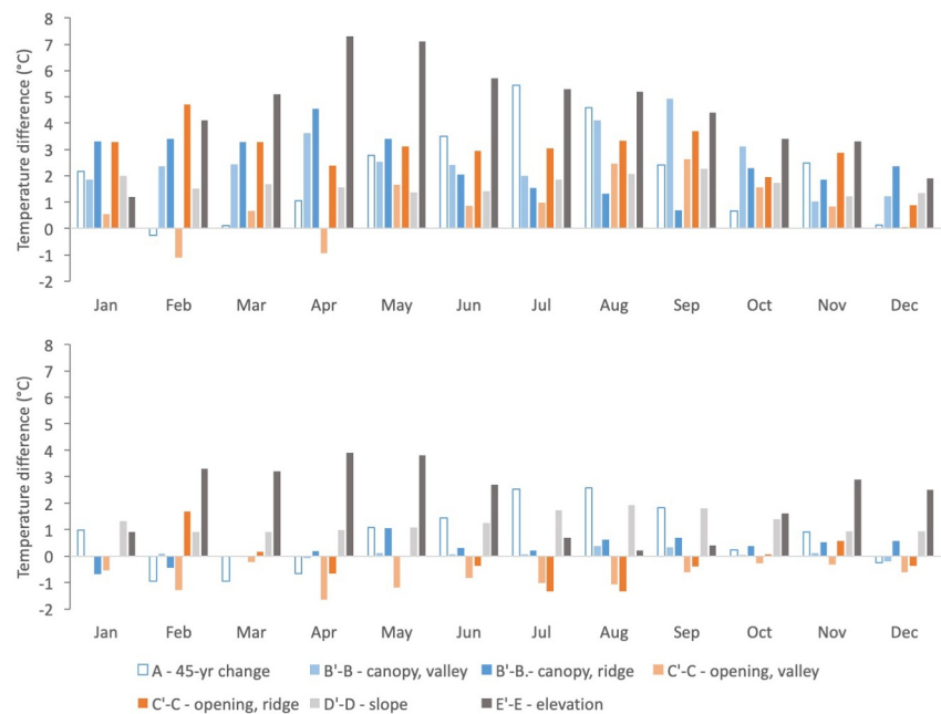
Figure 9. Long-term rates of temperature change exceed spatial temperature differences in the Andrews Forest in many months of the year. (a) Mean monthly T_{\max} and (b) mean monthly T_{\min} . Columns (from Figure 1) are A = 45-year total temperature change (Figure 3, Table S3N in Supporting Information S1) ( ^{\circ}\text{C}/\text{decade} times 4.5 decades, 1979–2023); B'-B = temperature at 36.5 m height in the canopy (B') minus at 1.5 m in the understory (B) of instrumented trees from trees in valley floor and ridge landscape positions, for 2016–2017 (Table S1 in Supporting Information S1); C'-C = temperature at 1.5 m in openings (C') versus at 1.5 m in the understory (C) of nearby forest in valley floor and ridge landscape positions, for 2016–2017 (Table S1 in Supporting Information S1); temperature in the forest understory on equator-facing slopes (D') versus polar-facing slopes (D) controlling for elevation (Figure 7); E'-E = temperature in the understory at low elevation (E') minus high elevation (E) ( ^{\circ}\text{C}/1,000 m) (Figure 7).
