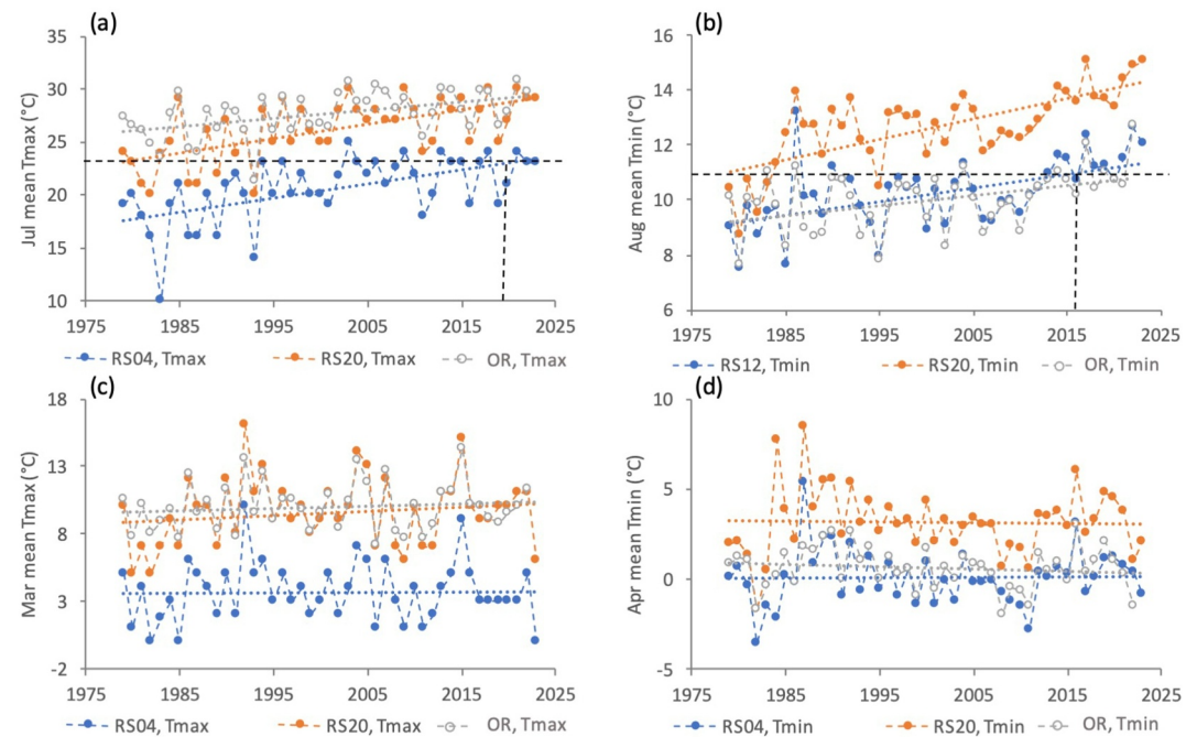
Figure 4. Comparison of temperature time series (1979–2023) in the coolest and warmest sites in the Andrews Forest and statewide average temperature for Oregon for selected months. (a, b) Examples of time series for months with the highest rates of temperature change: monthly T_{\max} in July (a) and T_{\min} in August (b). (c, d) Examples of time series for months with the lowest rates of temperature change: monthly T_{\max} in March (c) and T_{\min} in April (d). Plots also illustrate the strong correlations among time series of air temperature within the Andrews Forest and with statewide average temperature for Oregon (Table S4 in Supporting Information S1). Data sources: Daly et al. (2024), Menne et al. (2009).
