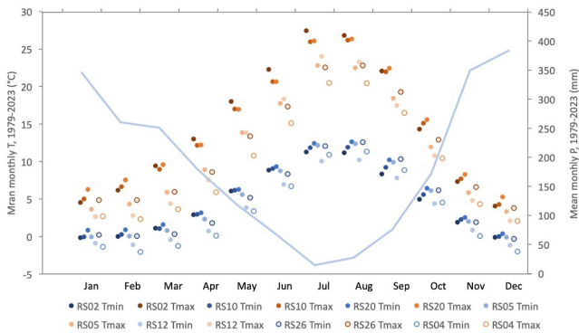
Figure 6. Mean monthly maximum ( T_{\max} ) and minimum ( T_{\min} ) air temperature and average diel temperature range at reference stands in the Andrews Forest, 1979–2023 (open and filled circles of different colors). For each month, reference stands are arranged from low to high elevation, left to right, dark to light shades. Elevations are: RS02—490 m, RS10—610 m, RS20—683 m, RS05—880 m, RS12—1,010 m, RS26—1040 m, RS04—1310 m (Table S2 in Supporting Information S1). Mean monthly precipitation (P, blue line), 1979–2023 at CS2 meteorological station (430 m). Data sources: Daly et al. (2019) and Daly et al. (2024).
